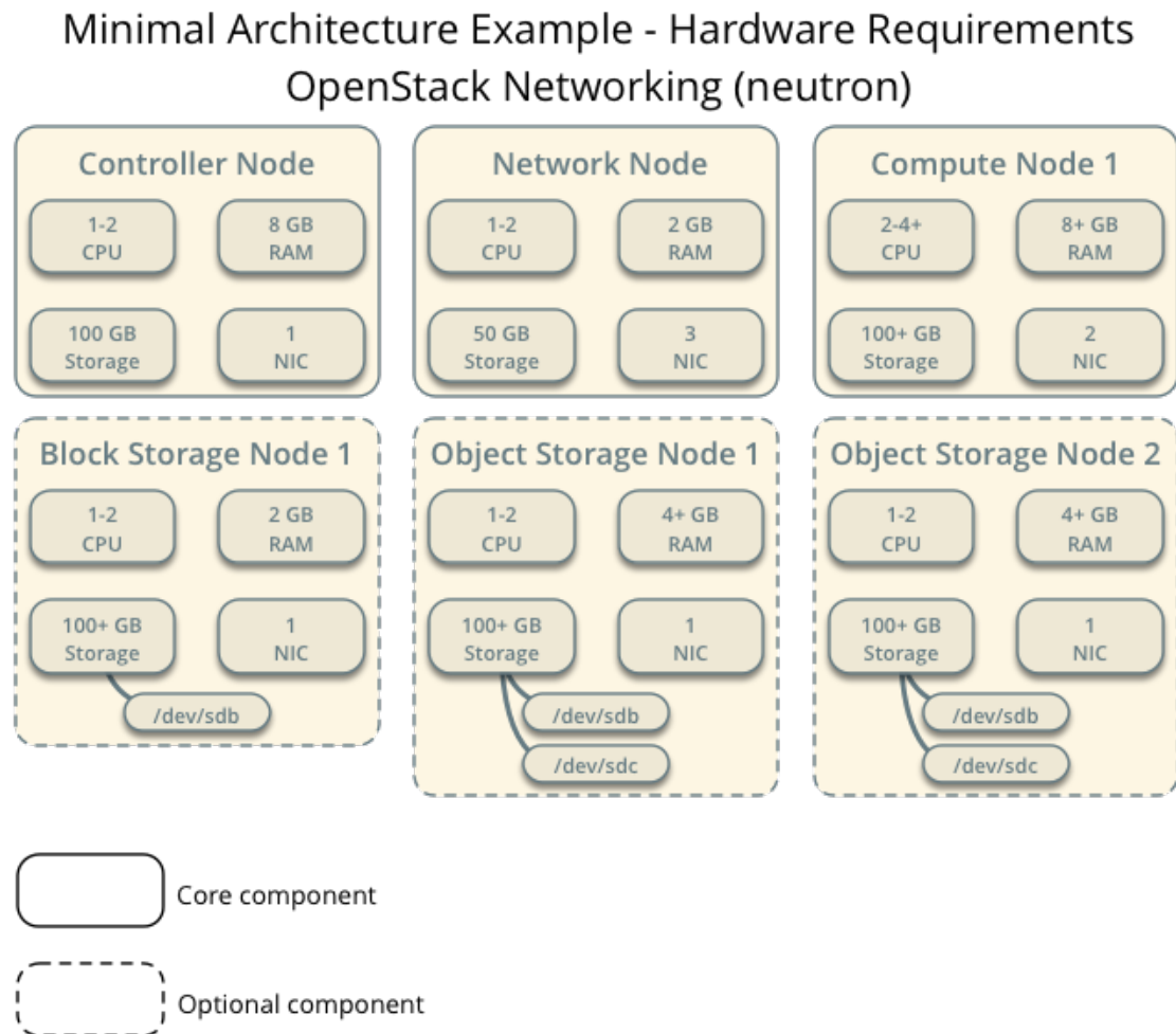
Figure 1.2. Minimal architecture example with OpenStack Networking (neutron)—Hardware requirements
